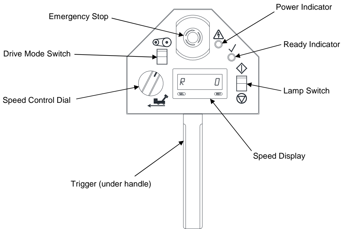
Fig. 10 Irradiator Module Control Panel
